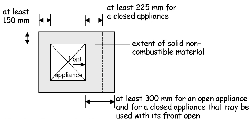
Plan of appliance on a hearth
