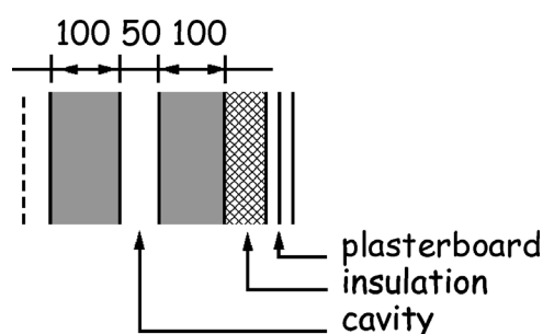
Figure 3.13 Wall constructions - Type A
