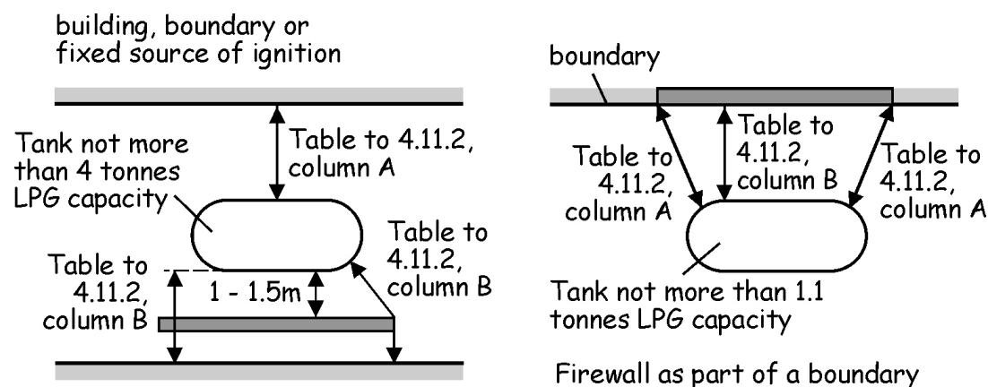
Figure 4.13 Separation or shielding of a LPG tank from a building, boundary or fixed source of ignition
